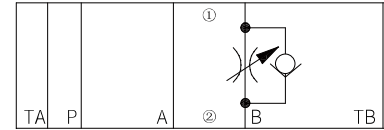
Model Z2FS10B-...-3XJ/...(meter-in control)
