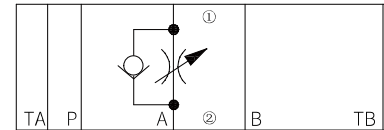
Model Z2FS10A-...-3XJ/...(meter-in control)
