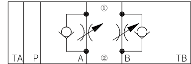
Model Z2FS10-...-3XJ/...(meter-in control)
